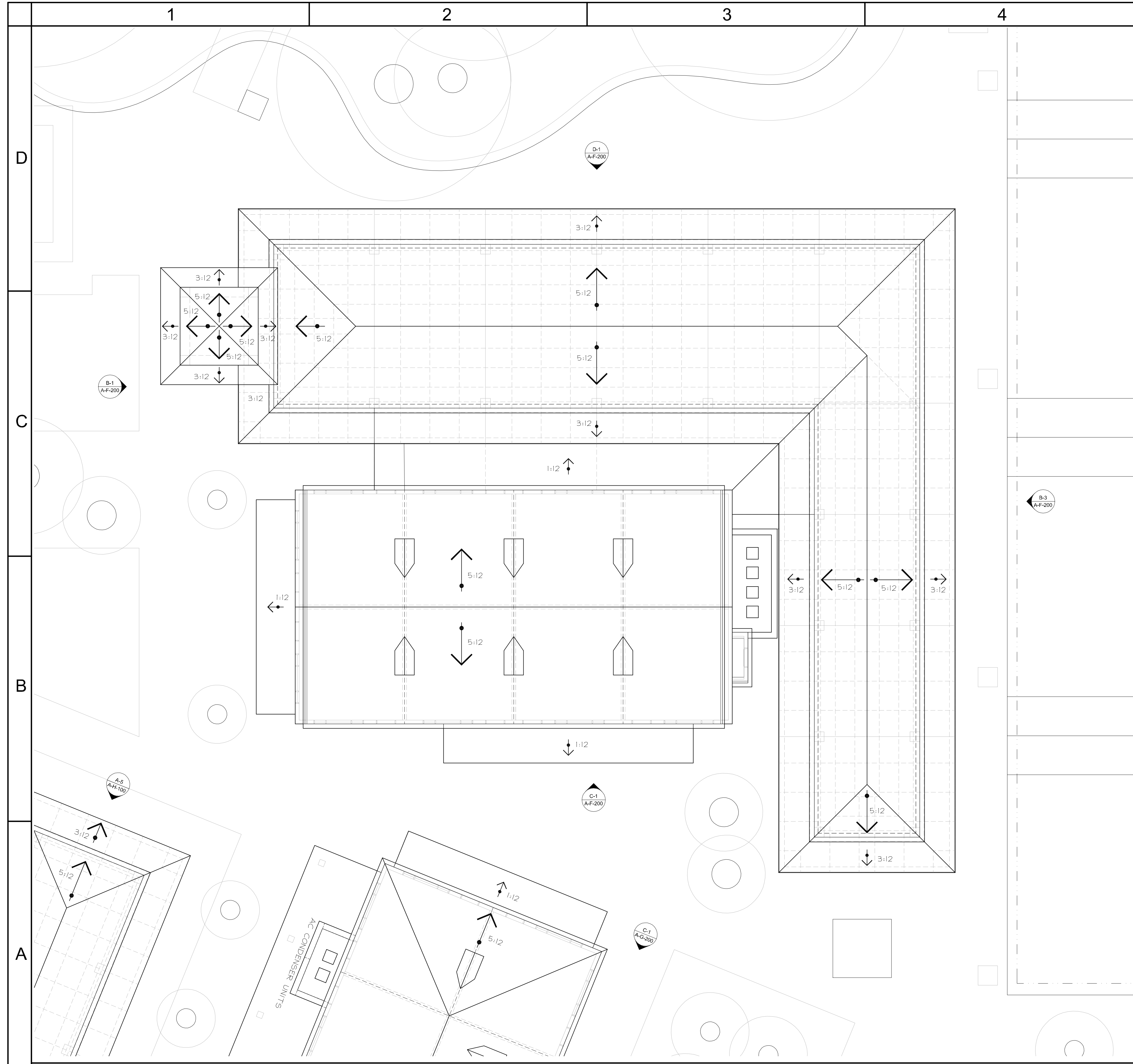
A-1 GROUND LEVEL PLAN
